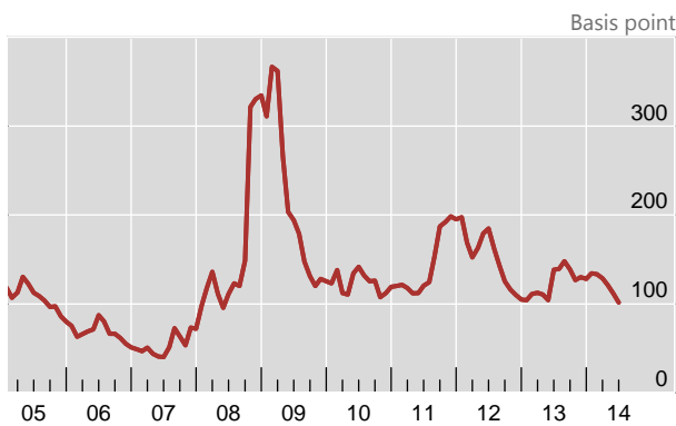
CDS spreads
