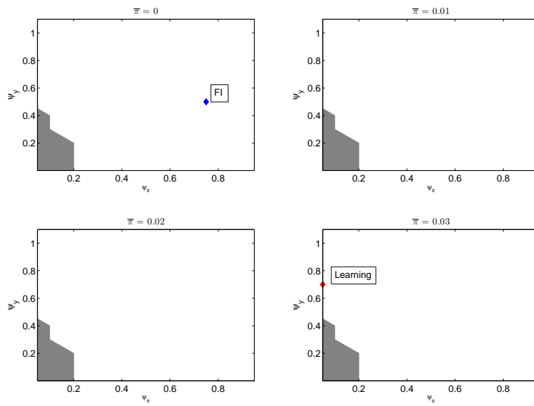
Figure 11: Nonexplosive region of H_1 when \bar{\pi} is known
