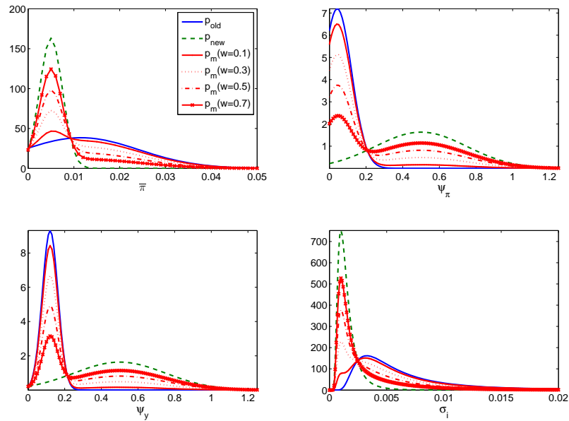
Figure A9: A family of mixture priors
